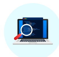
Manual Testing
