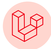
Laravel
