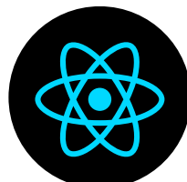
ReactJS
